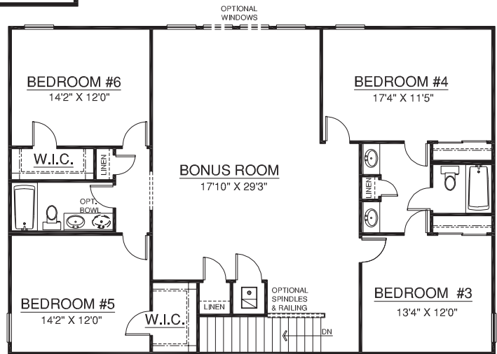
SECOND FLOOR PLAN w/ OPTIONAL 6th BEDROOM & BATH
