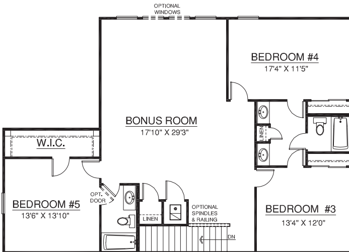
SECOND FLOOR PLAN w/ OPTIONAL SHARED BATH
