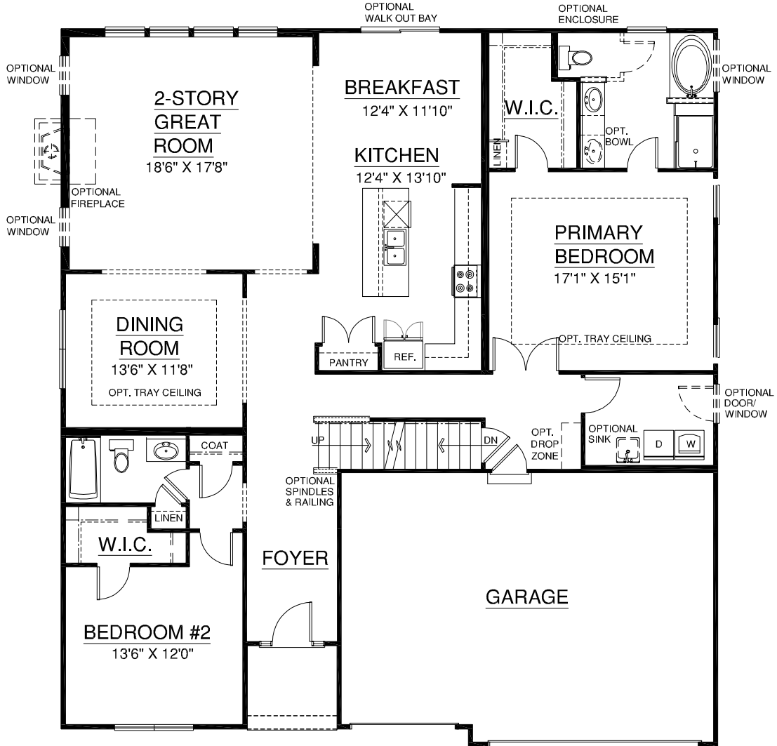
FIRST FLOOR PLAN W/ OPTIONAL 2-STORY GREAT ROOM
