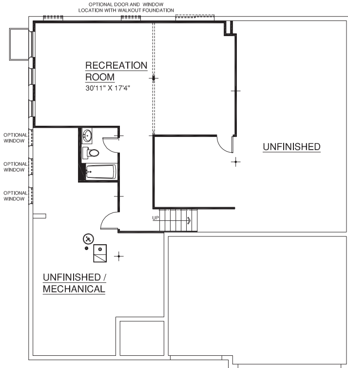
OPTIONAL FINISHED LOWER LEVEL #1
