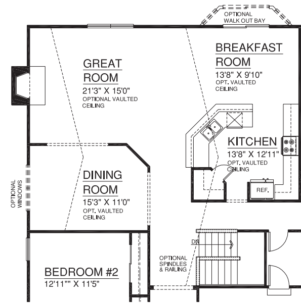
OPTIONAL FIRST FLOOR PLAN
