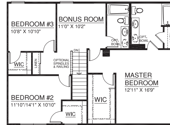
OPTIONAL SECOND FLOOR PLAN
