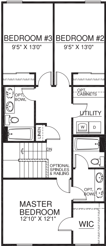
OPTIONAL SECOND FLOOR PLAN
