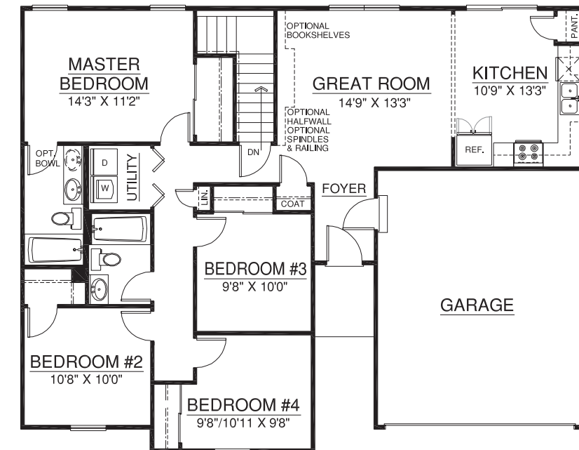
OPTIONAL FIRST FLOOR PLAN W/ 4TH BEDROOM
